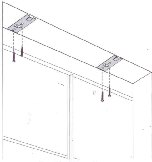
Inside Mount
