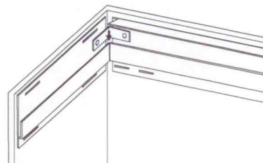
Secure return with corner brace
